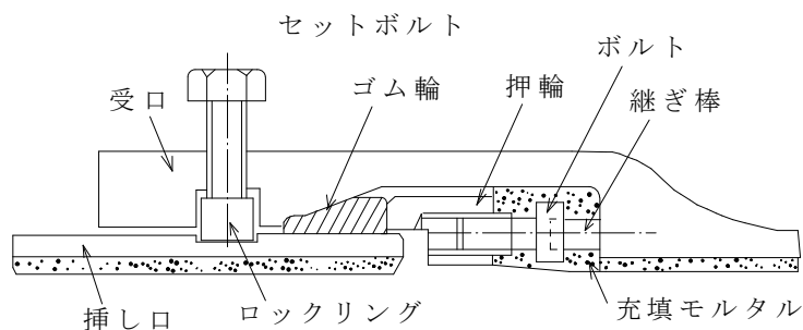
図ー5.6 U F 形管の接合
