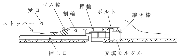
図ー5.4 U形管の結合
