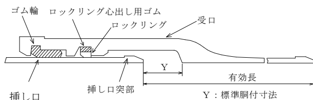
図ー5.11 NS形管の接合
